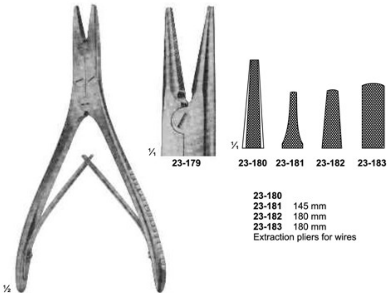
23-179 - 183 Round pliers 180 mm
