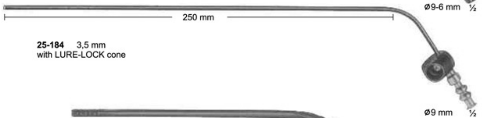
25-185 LANDOLT with finger cut-off and stylet, can be sterilized in an autoclave up to 3 bar (143 °C)
